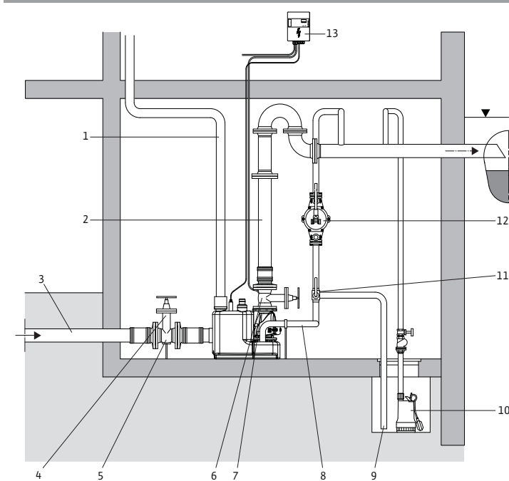
Fig. 12: Installation example
