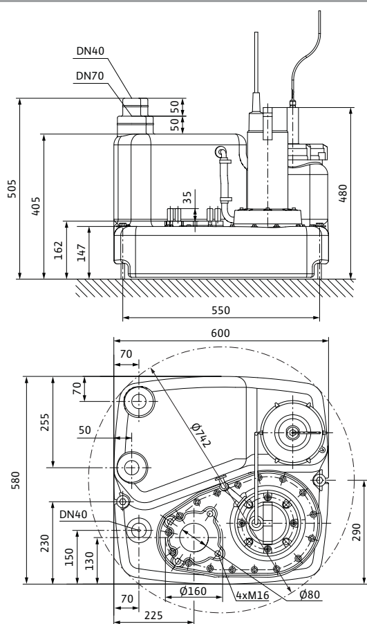
Fig. 2: Installation plan
