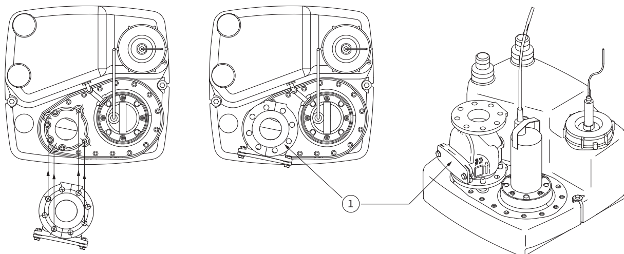
Fig. 5: Installation/alignment of the non-return valve
