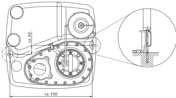
Fig. 4: Buoyancy safeguard
