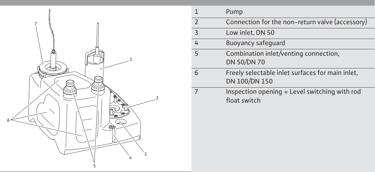
Fig. 1: Description of the unit
