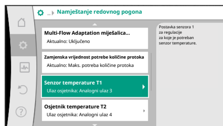
Fig. 62: Multi-Flow Adaptation miješalica: Osjetnik temperature
