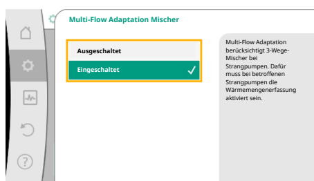
Fig. 61: Multi-Flow Adaptation Mischer
