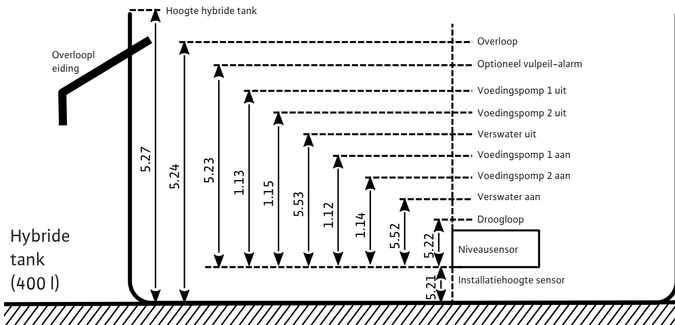
Fig. 25: Instelparameters hybride tank
