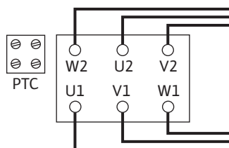
Fig. 14: Controlo Y-Δ
