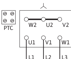
Fig. 15: Y-tilkobling
