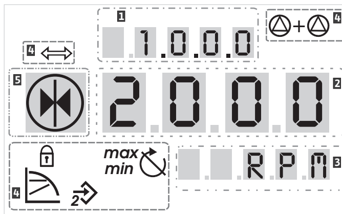
Fig. 36: Displaylayout
