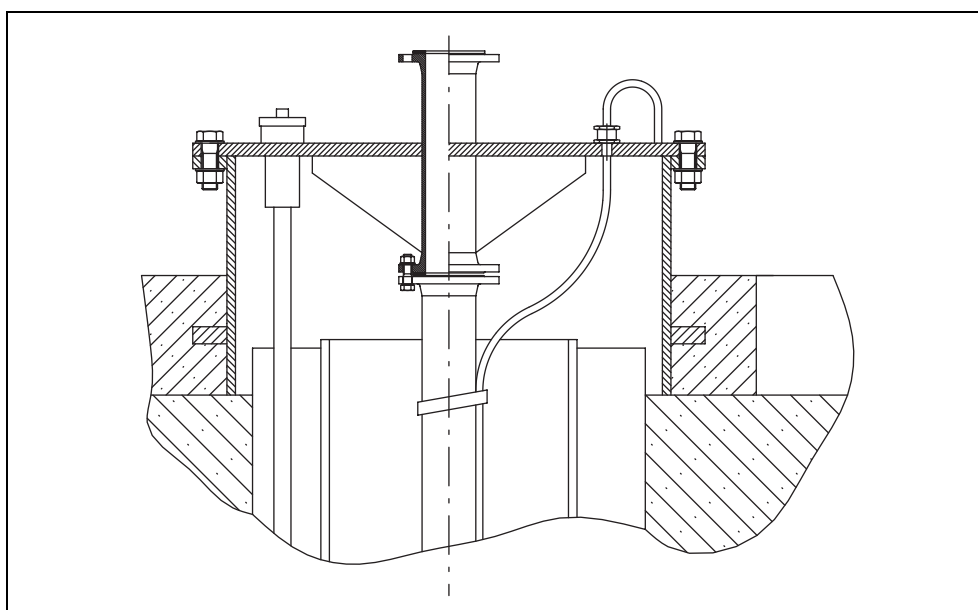
Obr. 5-3: Obrubeň studny
