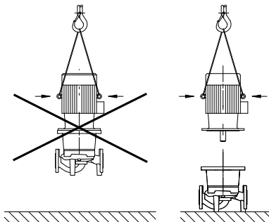
Fig. 35: Transport motora
