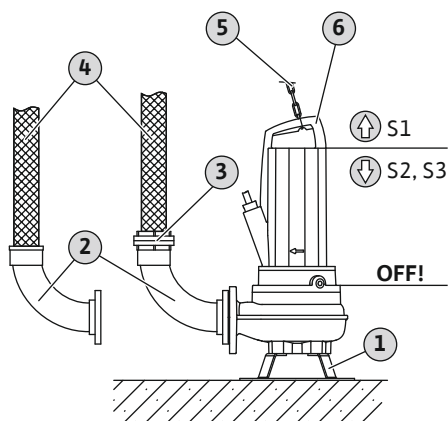
Fig. 5: Installation immergée transportable
