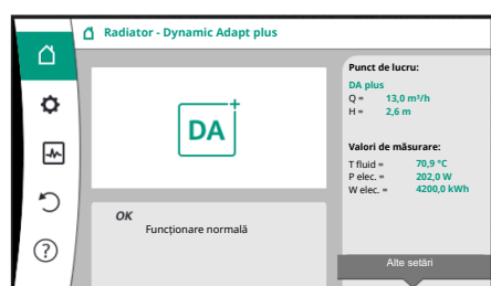
Fig. 32: Meniu principal
