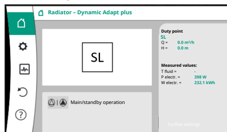
Fig. 64: Home screen en twin-head pump partner without a mounted differential pressure sensor
