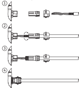
Fig. 24: Shield clamp
