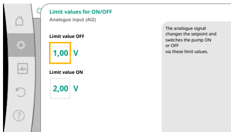
Fig. 79: Limit values for ON/OFF control through analogue signal
