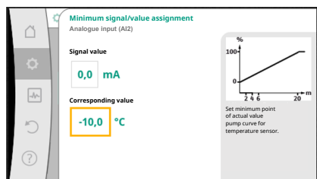
Fig. 85: Minimum signal/value assignment, actual value sensor
