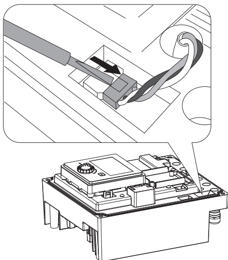
Fig. 104: Loosen the connection cable of the module fan
