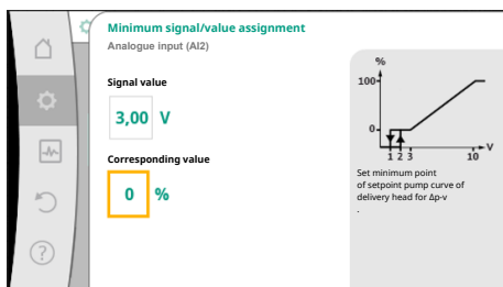
Fig. 80: Minimum signal/value assignment
