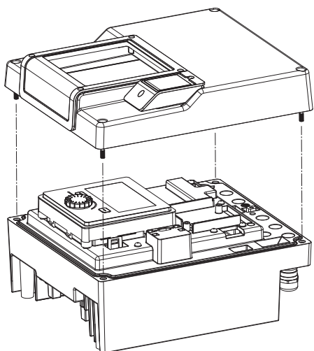
Fig. 103: Open the cover of the electronic module
