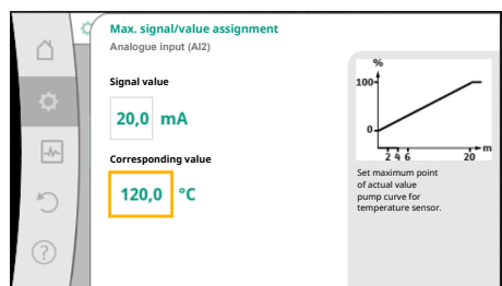
Fig. 86: Maximum signal/value assignment, actual value sensor
