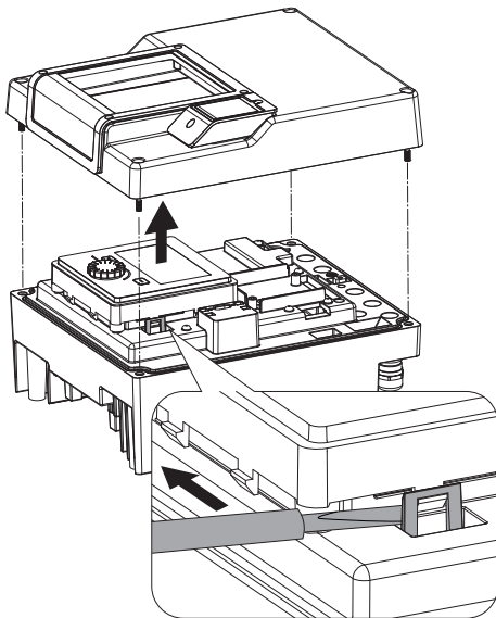
Fig. 107: Dismantle the module cover; release the display and control unit from the locking mechanism
