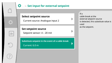
Fig. 82: Substitute setpoint in the event of a cable break
