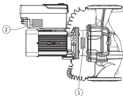
Fig. 2: Rating plates
