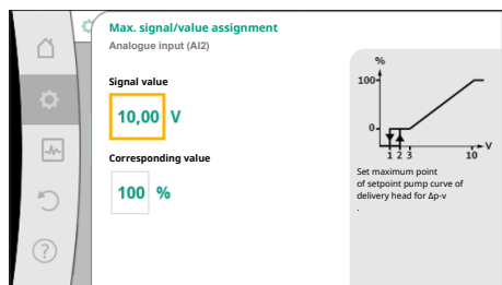
Fig. 81: Max. signal/value assignment
