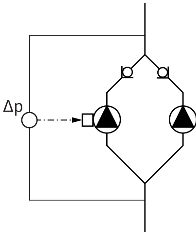
Fig. 17: Example – differential pressure sensor connection in y-pipe installation
