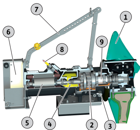
Fig. 2: Panoramic view of a submersible motor agitator
