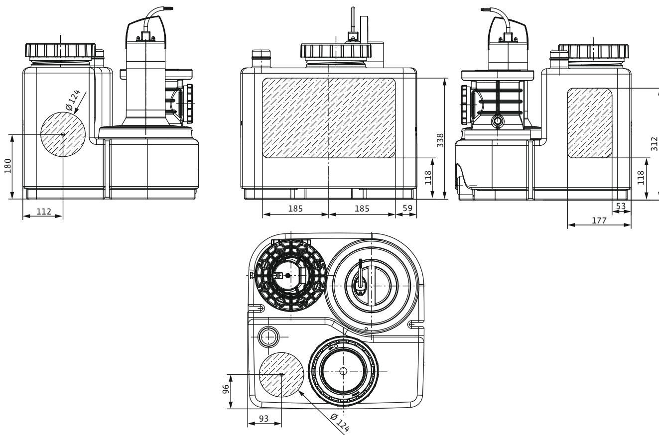
Fig. 4: Inlet areas
