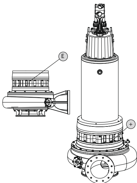
Fig. 20: Wentellager nasmeren FKT 50.1, 57, 63.1
