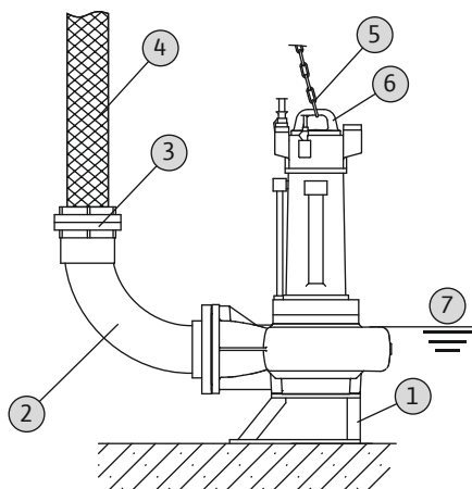
Fig. 9: Vådinstallation, transportabel
