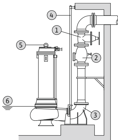
Fig. 8: Natte opstelling, stationair
