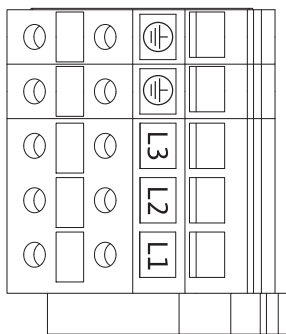
Fig. 25: Elektros gnybtai (Tinklo prijungimo gnybtai)
