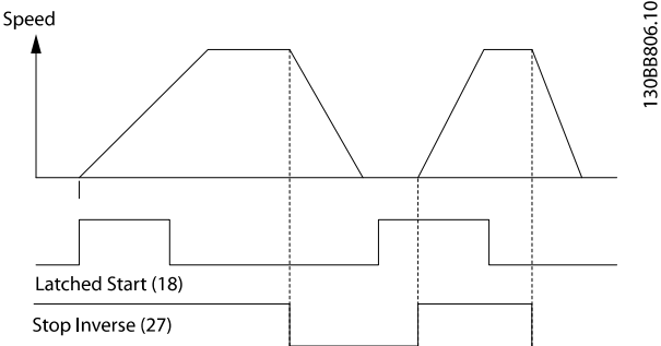
Illustration 6.3 Pulsstart/inverteret stop
