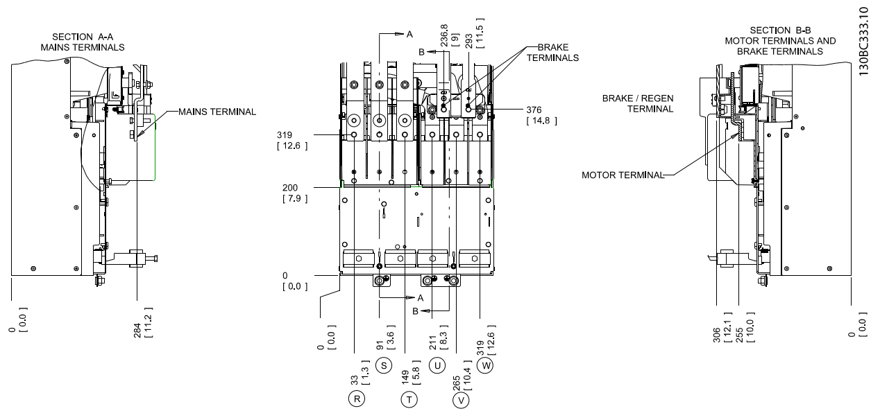
Illustration 4.9 Klemmeplaceringer, D4h
