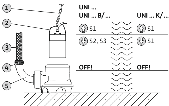
Fig. 6: Vådinstallation, transportabel
