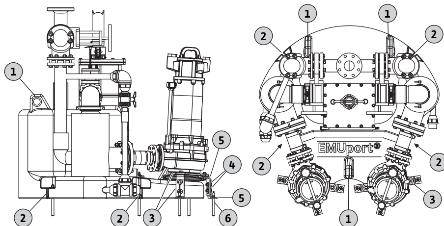
Fig. 3: Installation de la station de relevage
