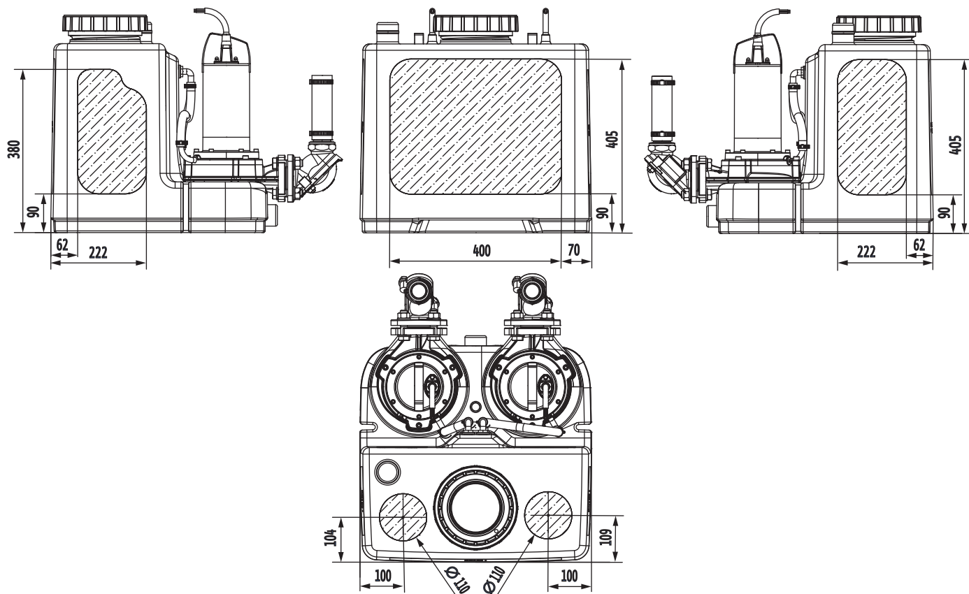
Fig. 4: Inlet areas
