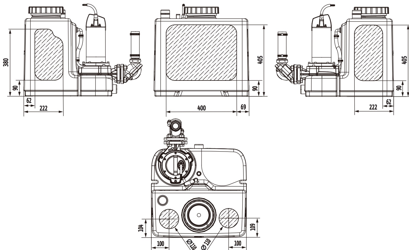
Fig. 4: Inlet areas
