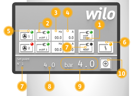
PLC - HMI
