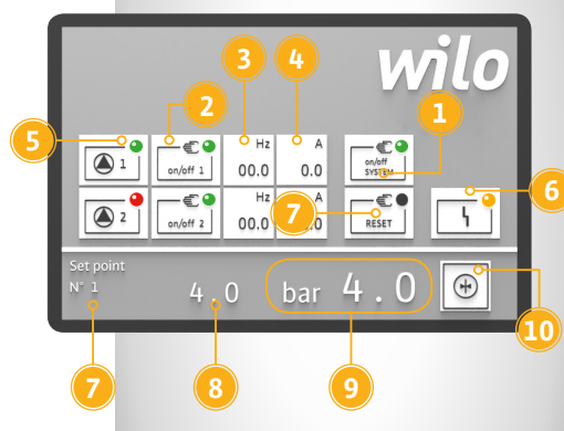
PLC - HMI
