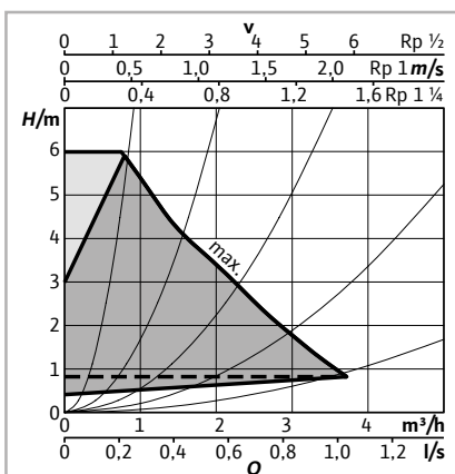
Stratos PICO 15, 25, 30/0,5-6
