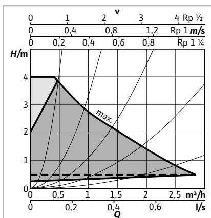
Stratos PICO 15, 25, 30/0,5-4
