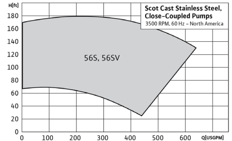
Scot Classic Cast Stainless Steel, Close-Coupled Pumps Models: 56S- NPT or Victaulic fittings
