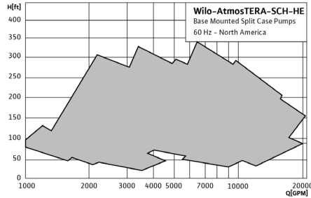
Wilо-Atmos TERA-SCH-HE Base Mounted Split Case Pumps
