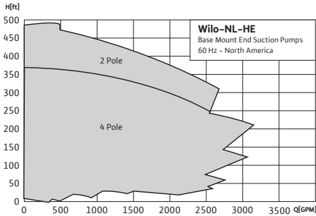
Wilо-NL-HE Base Mounted End Suction Pumps
