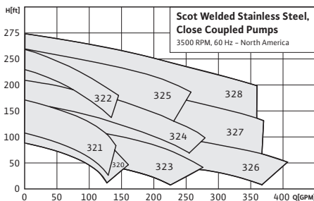
Scot Welded Stainless Steel, Close-Coupled Pumps, 3500 RPM Models: 320 Series
