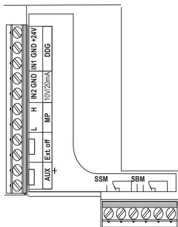
Fig. 26: Valdymo gnybtai
