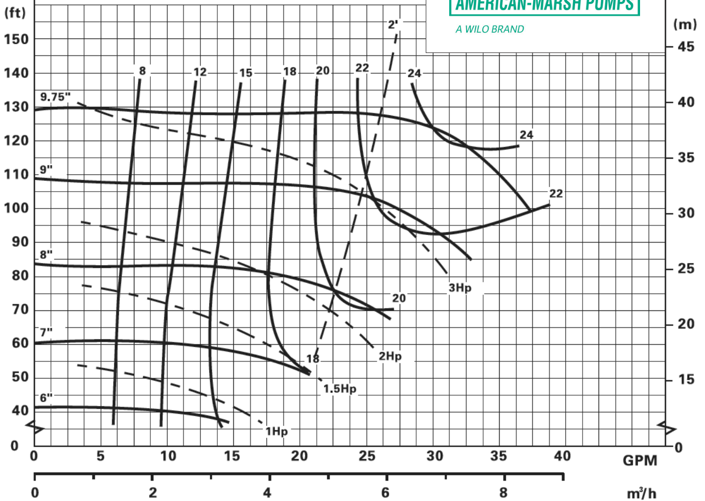
CHEMICAL PROCESS PUMP CHARACTERISTICS
