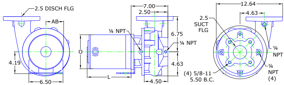
DRAWING DEPICTS 56C ODP MOTOR ALL DIMENSIONS IN INCHES
