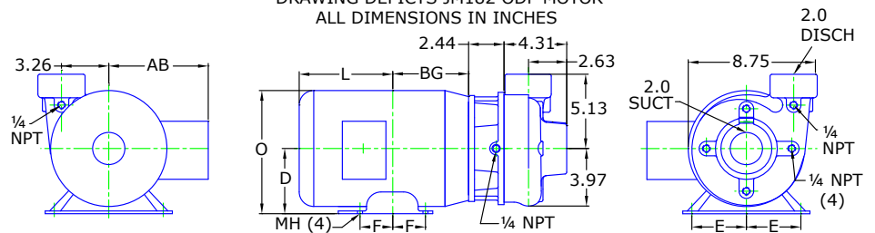
DRAWING DEPICTS JM182 ODP MOTOR ALL DIMENSIONS IN INCHES
