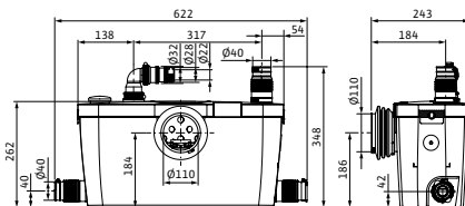
HISEWLIFT 3-35
