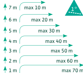
HIDRAINLIFT 3-37
