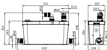
HIDRAINLIFT 3-35, 3-37
