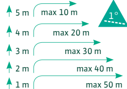
HIDRAINLIFT 3-35
