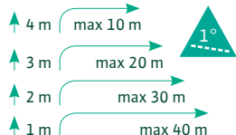
HIDRAINLIFT 3-24
