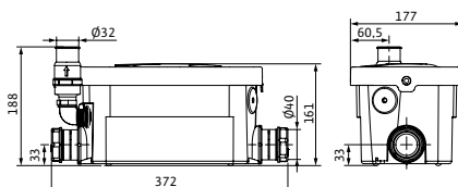
HIDRAINLIFT 3-24
