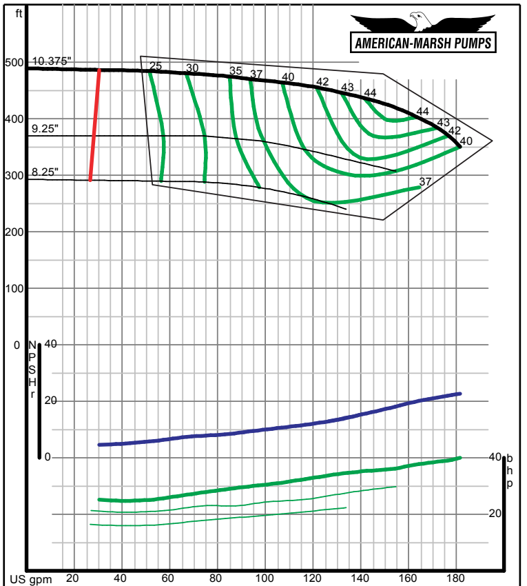
American-Marsh Pumps Size: 1.25x2-10 SREM Speed: 3500 rpm
