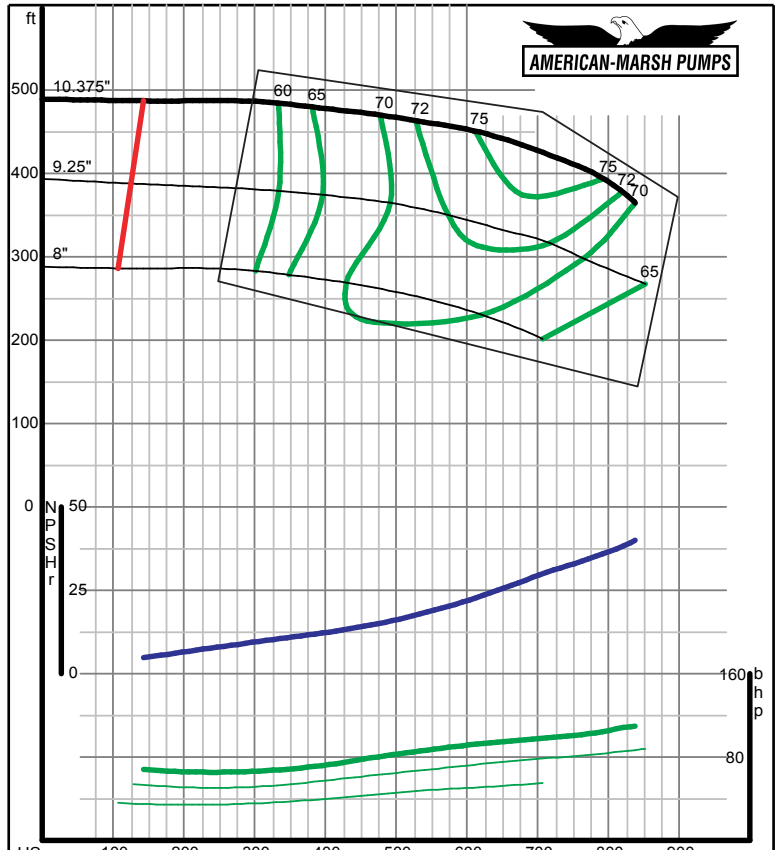
American-Marsh Pumps Size: 2.5x3-10 SREM Speed: 3500 rpm
