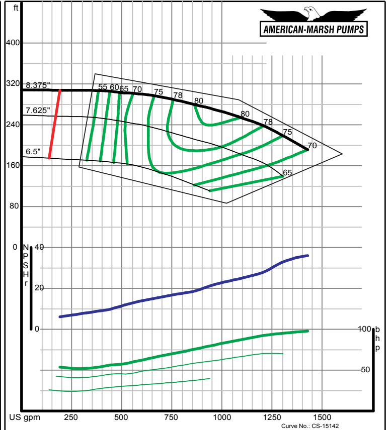
American-Marsh Pumps Size: 3x4-8 SREM Speed: 3500 rpm
