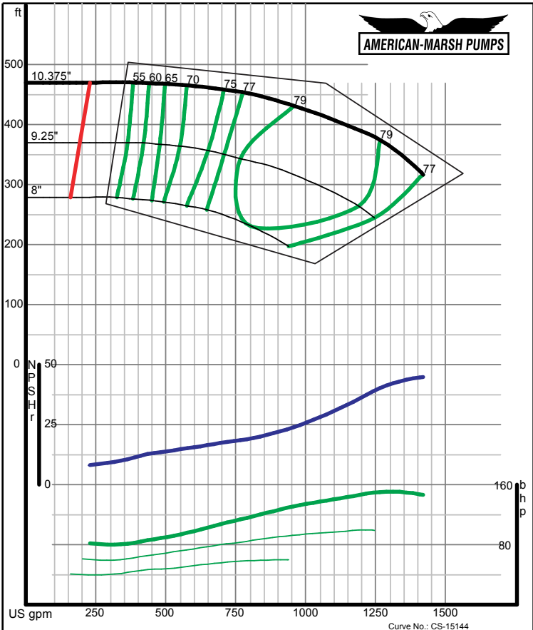
American-Marsh Pumps Size: 3x4-10 SREM Speed: 3500 rpm
