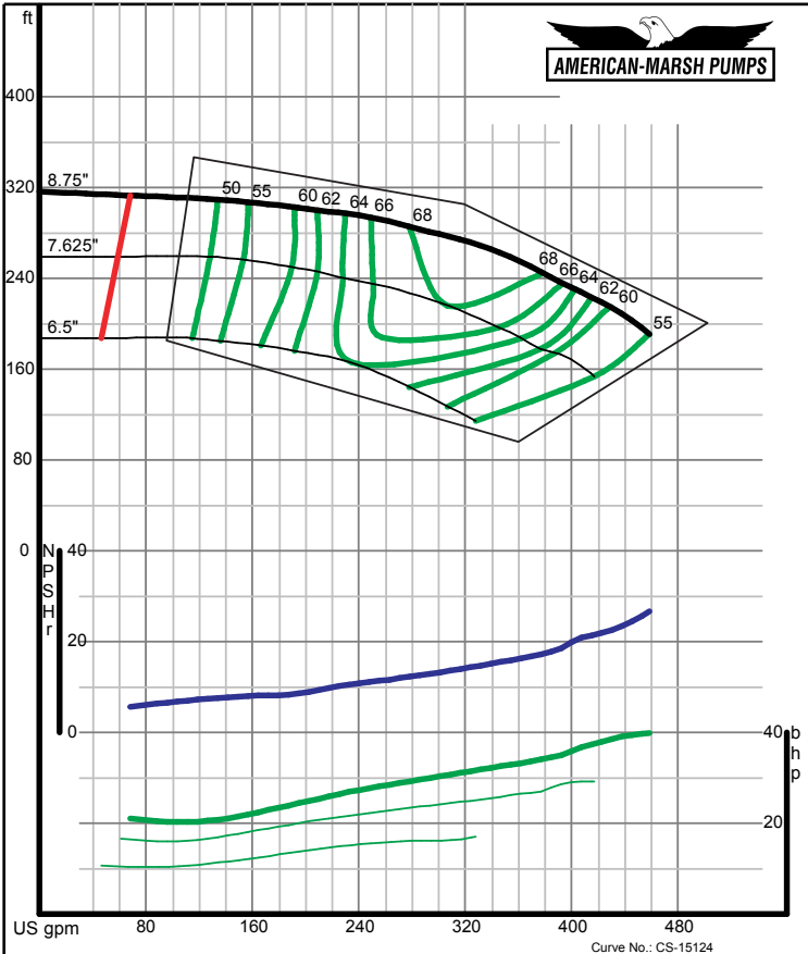
American-Marsh Pumps Size: 2x2.5-8 SREM Speed: 3500 rpm 09/03/02
