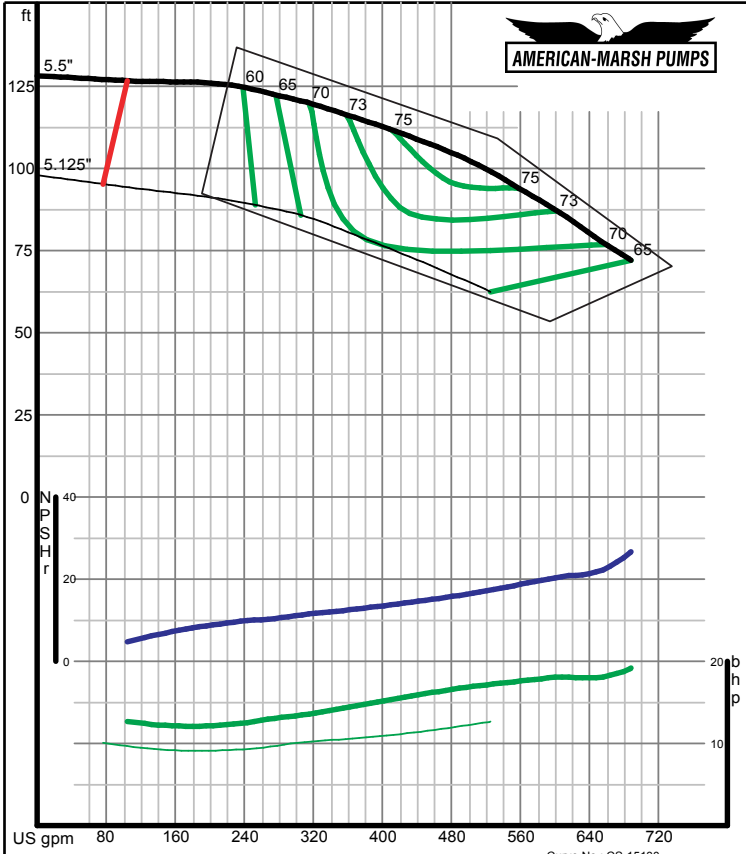
American-Marsh Pumps Size: 2.5x3-5 SREM Speed: 3500 rpm
