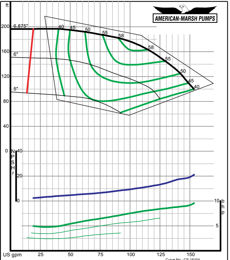
American-Marsh Pumps Size: 1.25x2-7 SREM Speed: 3500 rpm
