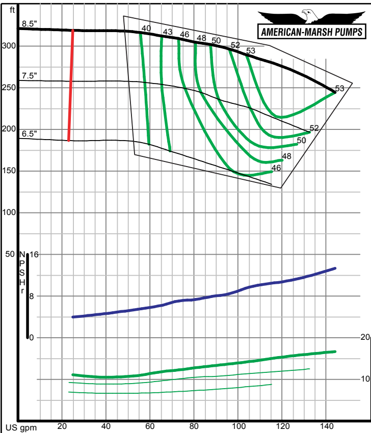
American-Marsh Pumps Size: 1.25x2-8 SREM Speed: 3500 rpm
