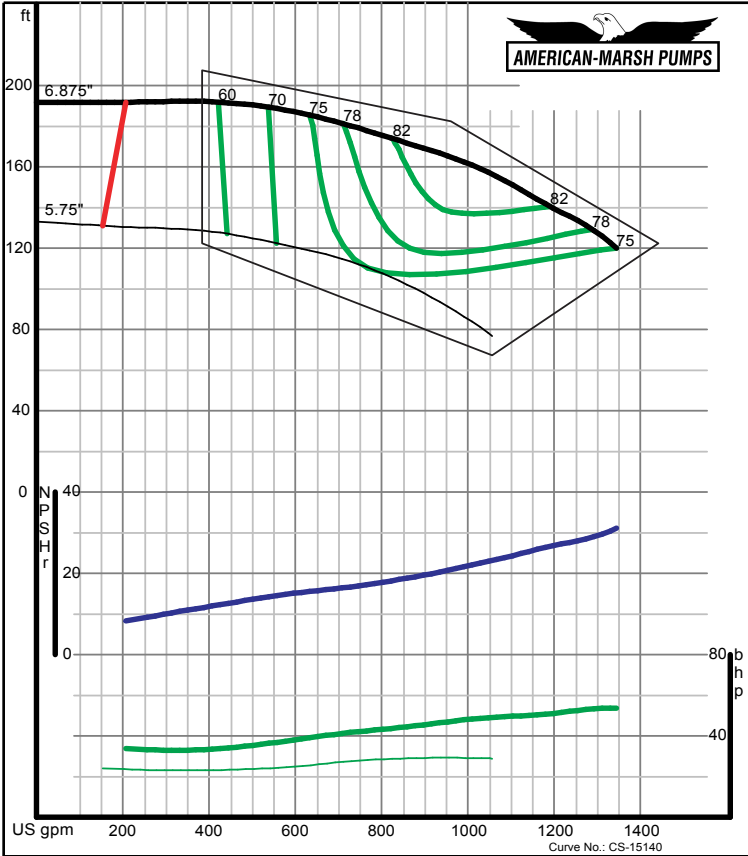
American-Marsh Pumps Size: 3x4-7 SREM Speed: 3500 rpm
