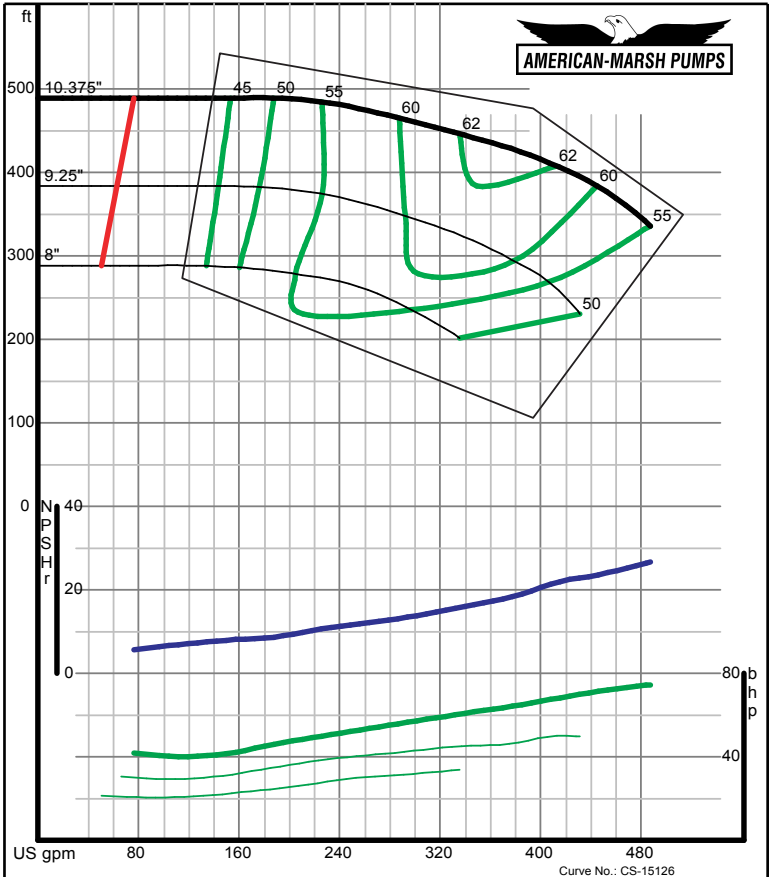
American-Marsh Pumps Size: 2x2.5-10 SREM Speed: 3500 rpm 09/03/02
