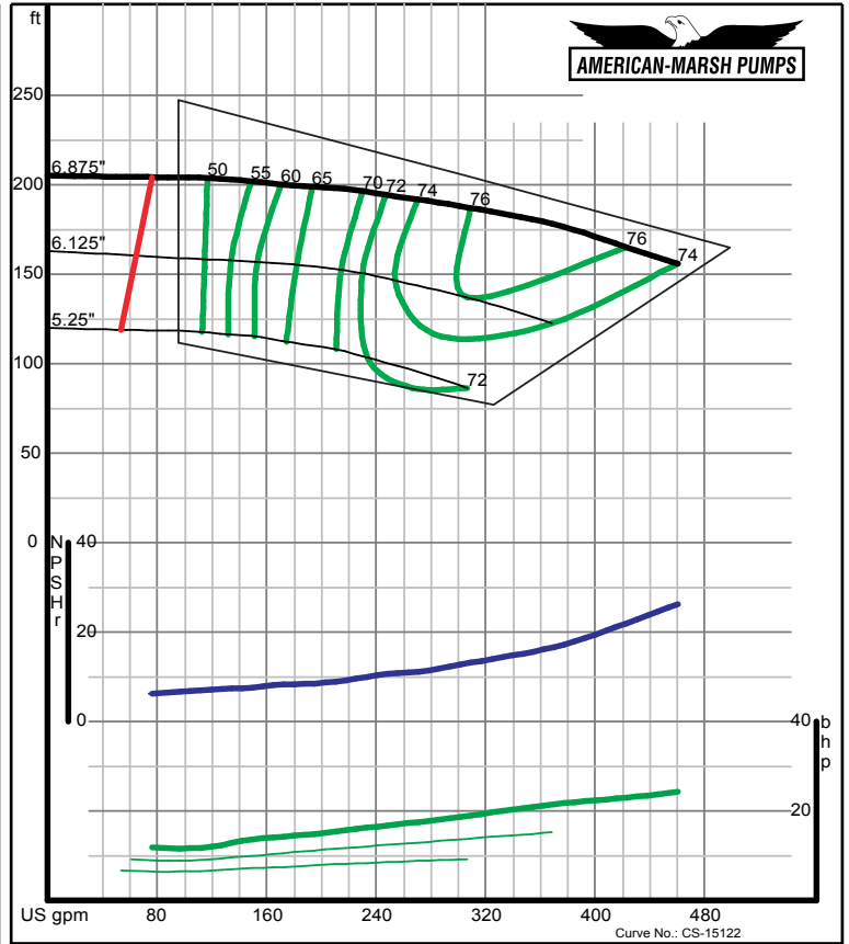
American-Marsh Pumps Size: 2x2.5-7 SREM Speed: 3500 rpm 09/03/02
