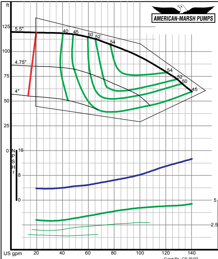
American-Marsh Pumps Size: 1.25x2-5 SREM Speed: 3500 rpm
