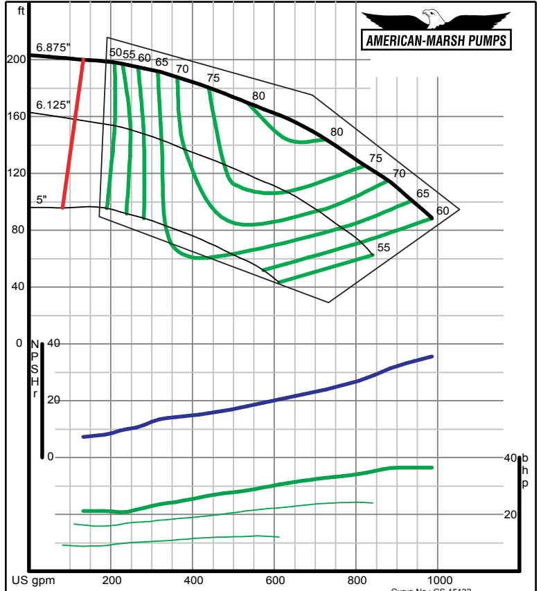
American-Marsh Pumps Size: 2.5x3-7 SREM Speed: 3500 rpm
