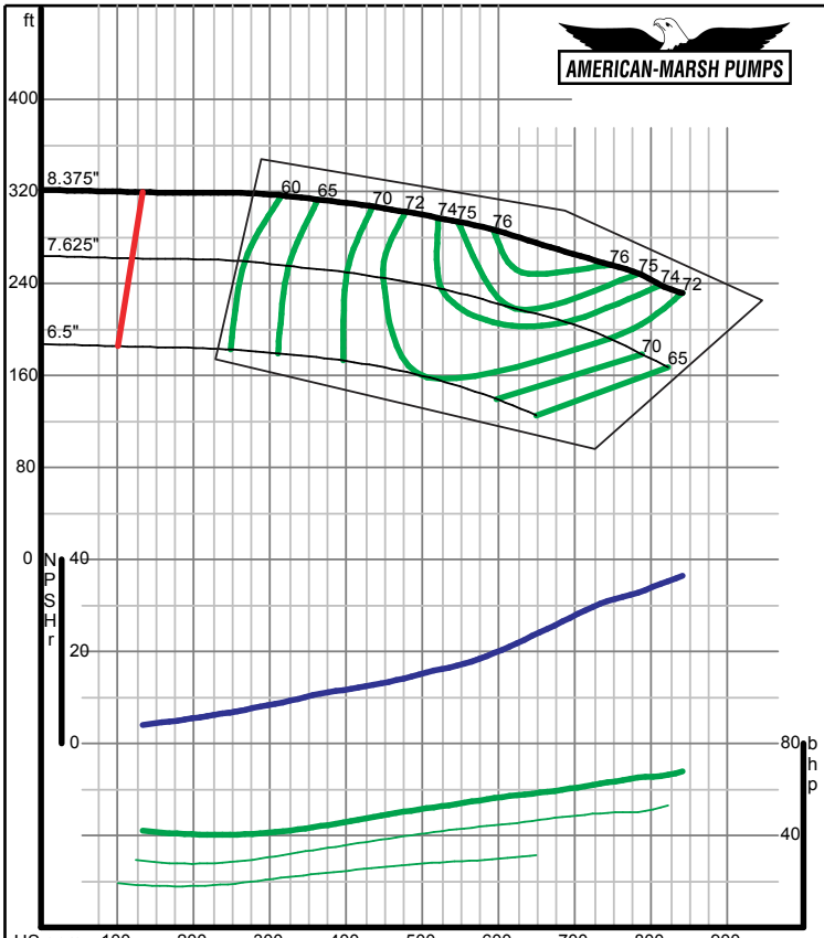
American-Marsh Pumps Size: 2.5x3-8 SREM Speed: 3500 rpm
