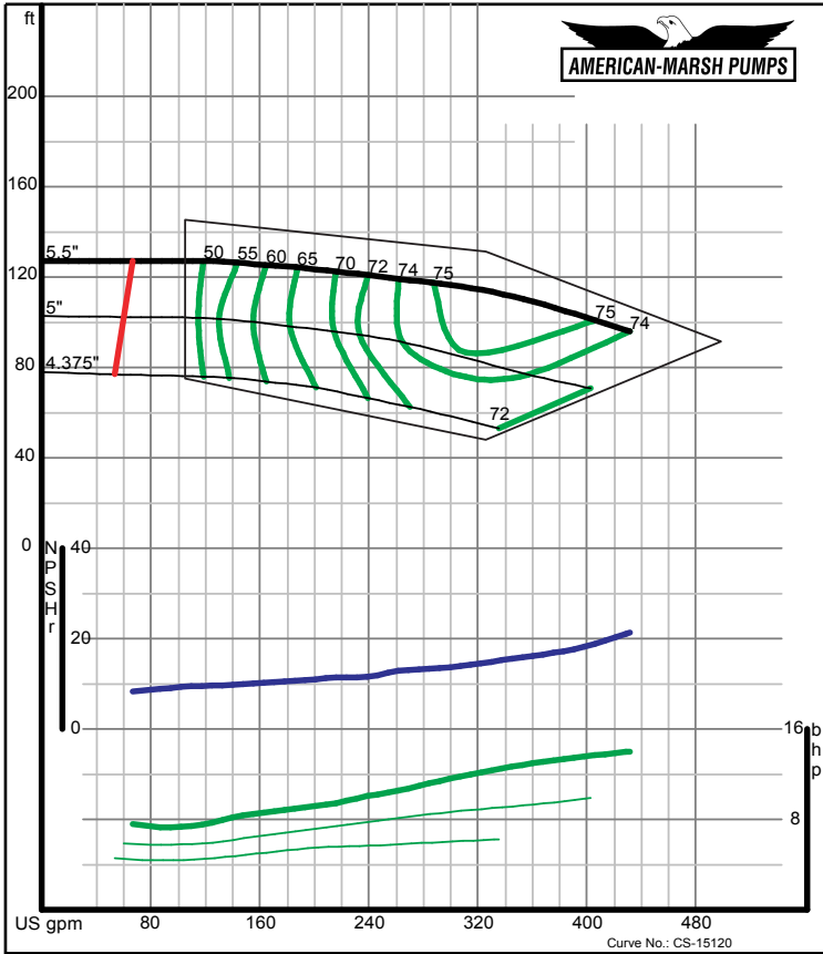
American-Marsh Pumps Size: 2x2.5-5 SREM Speed: 3500 rpm 09/03/02
