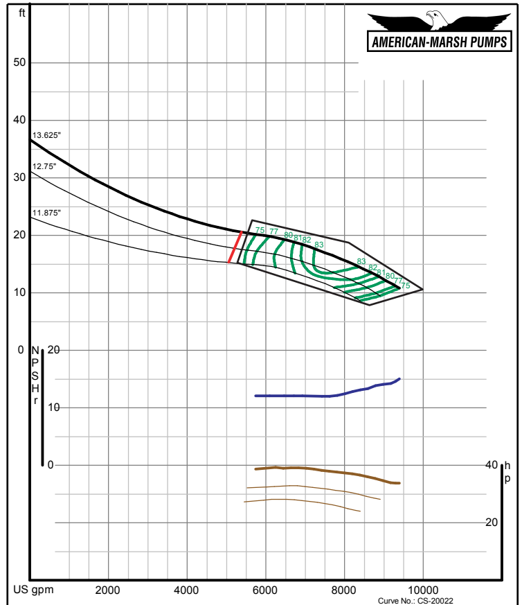
American-Marsh Pumps Size: 20MFM 08/01/05 Speed: 590 rpm Curve No.: CS-20022
