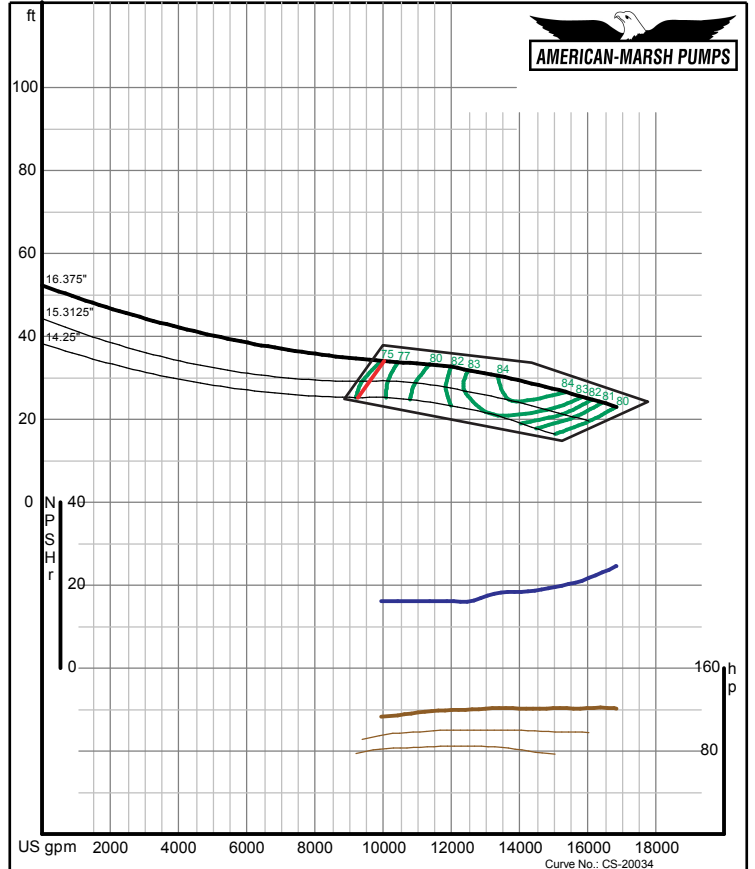
American-Marsh Pumps 08/01/05 Size: 24MFP Speed: 590 rpm
