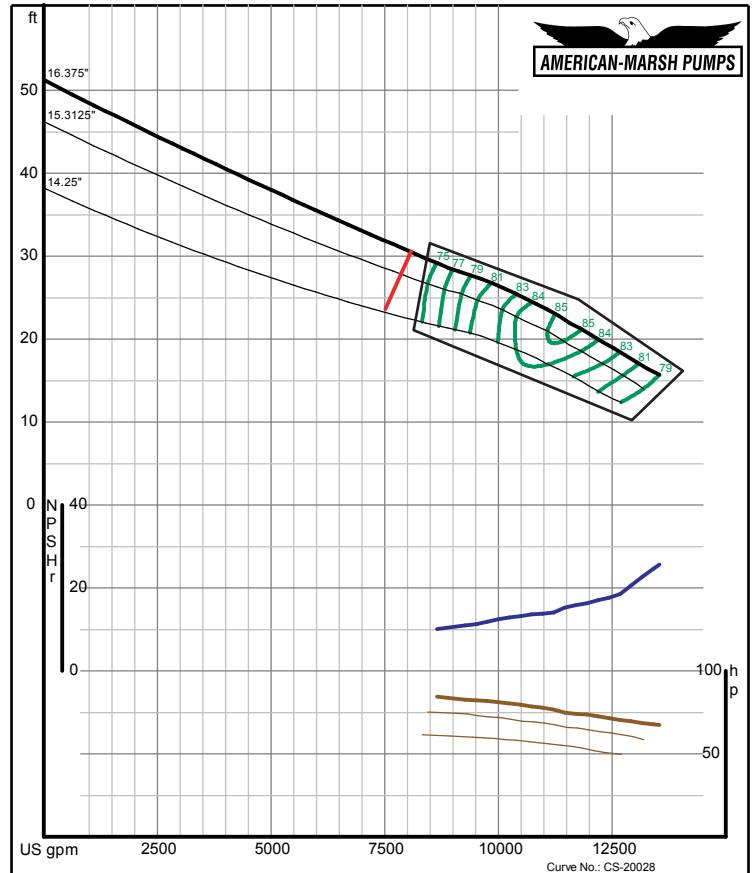
American-Marsh Pumps Size: 24MFL 08/01/05 Speed: 590 rpm Curve No.: CS-20028
