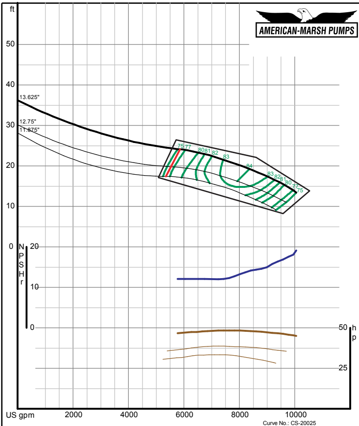
American-Marsh Pumps Size: 20MFP 08/01/05 Speed: 590 rpm Curve No.: CS-20025
