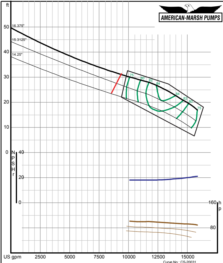
American-Marsh Pumps 08/01/05 Size: 24MFM Speed: 590 rpm
