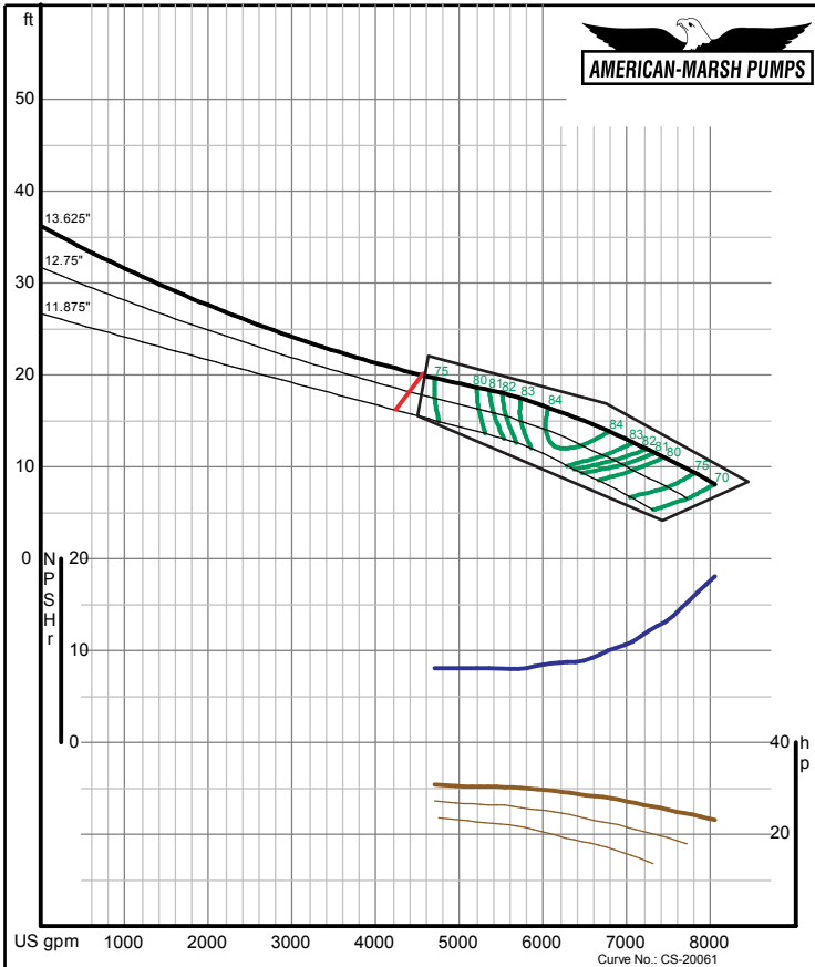
American-Marsh Pumps Size: 20MFL 08/01/05 Speed: 590 rpm Curve No.: CS-20061
