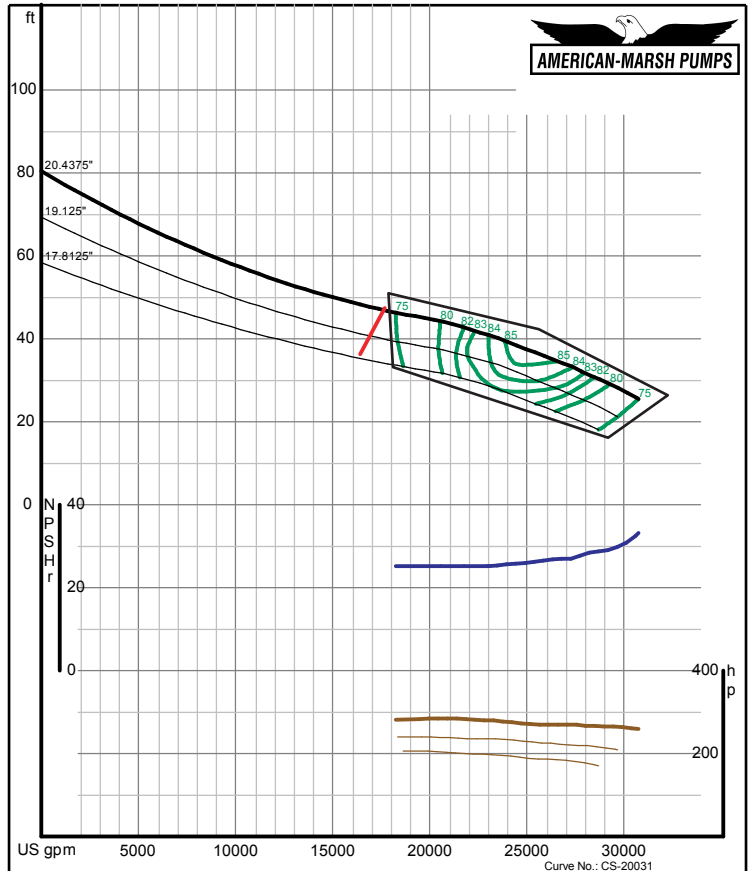
American-Marsh Pumps 08/01/05 Size: 30MFM Speed: 590 rpm
