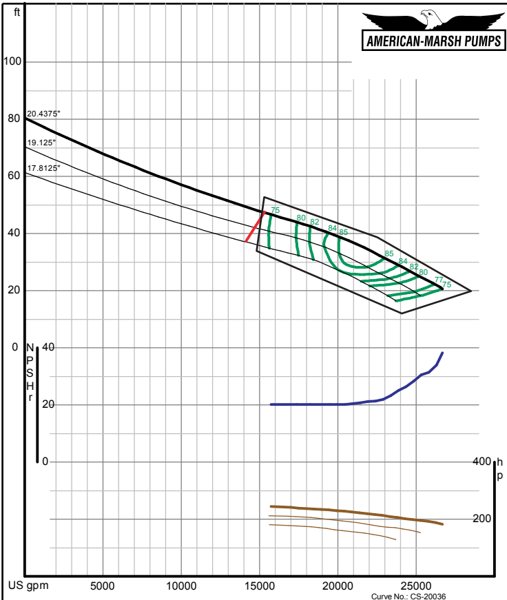
American-Marsh Pumps 08/01/05 Size: 30MFL Speed: 590 rpm
