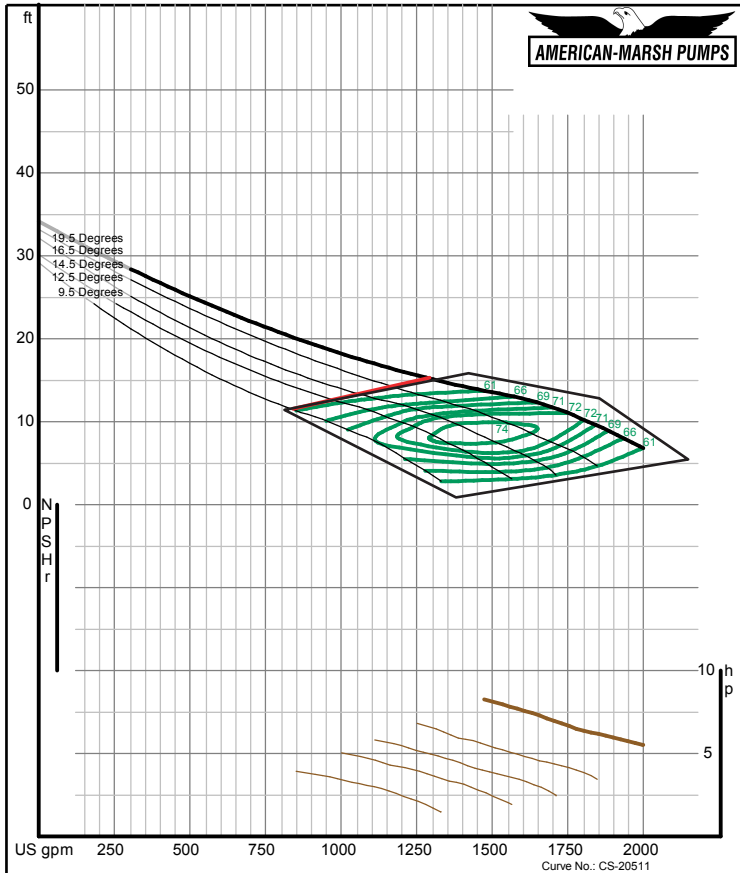
American-Marsh Pumps Size: 8AJ 08/01/05 Speed: 1750 rpm
