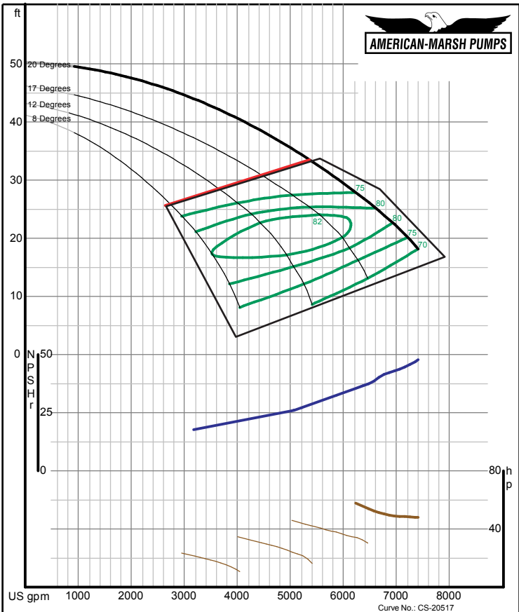
American-Marsh Pumps Size: 12AJ 08/01/05 Speed: 1750 rpm
