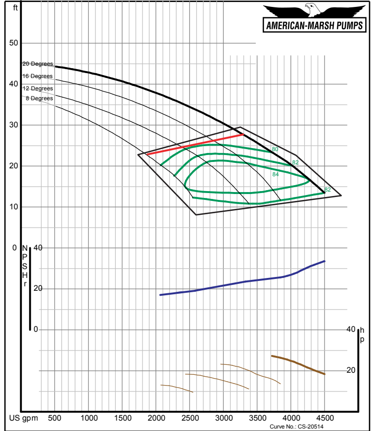
American-Marsh Pumps Size: 10AJ 08/01/05 Speed: 1750 rpm
