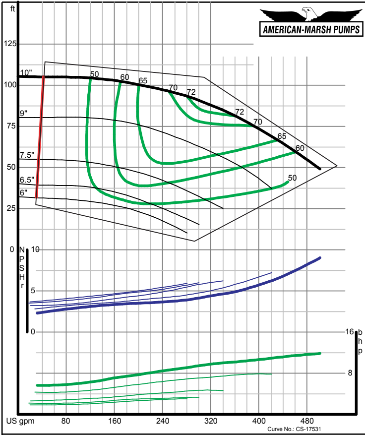
American-Marsh Pumps Size: 2L3X4-10/OP Speed: 1750 rpm 05/18/04
