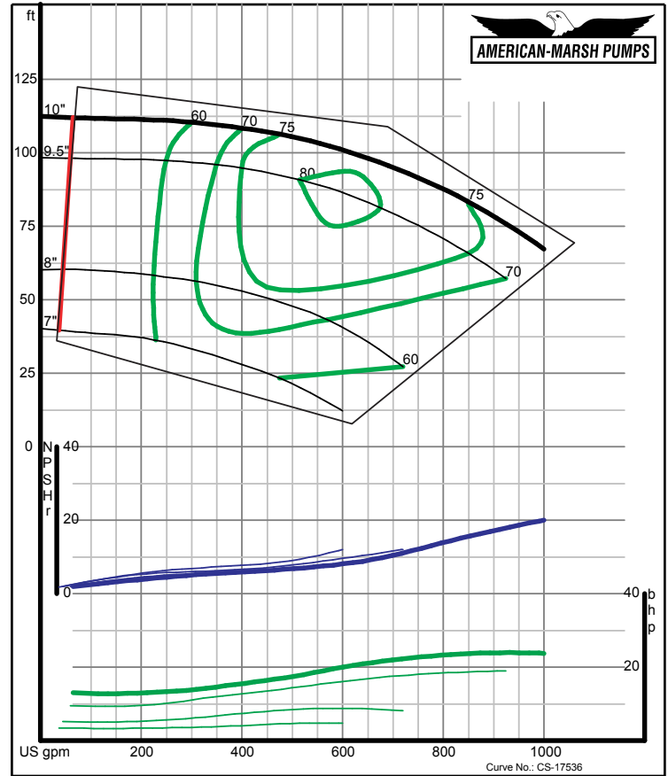
American-Marsh Pumps Size: 2L4X6-10/OP Speed: 1780 rpm 05/18/04
