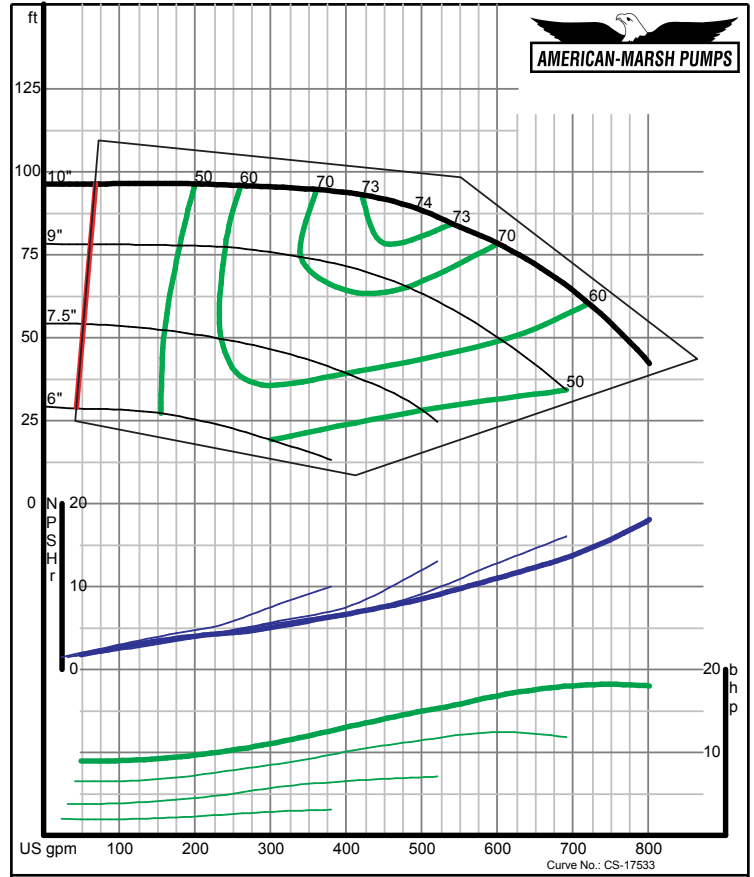
American-Marsh Pumps Size: 2L3X4-10H/OP Speed: 1750 rpm 05/18/04
