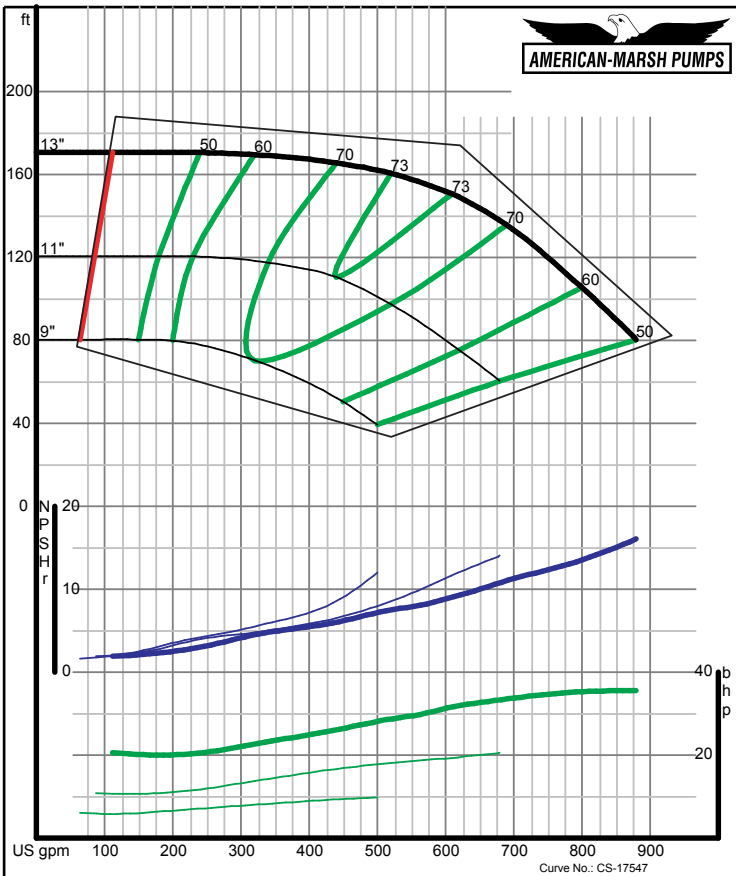
American-Marsh Pumps Size: 2L3X4-13/OP Speed: 1750 rpm 05/18/04
