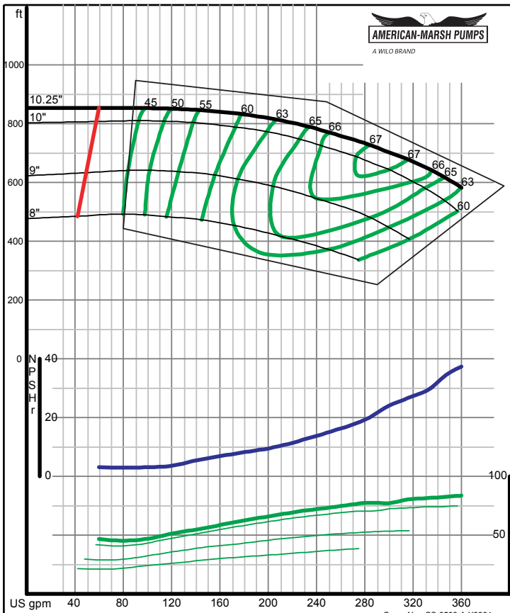
American-Marsh Pumps Size: 2x3-10 HH 2 stg Speed: 3500 rpm
