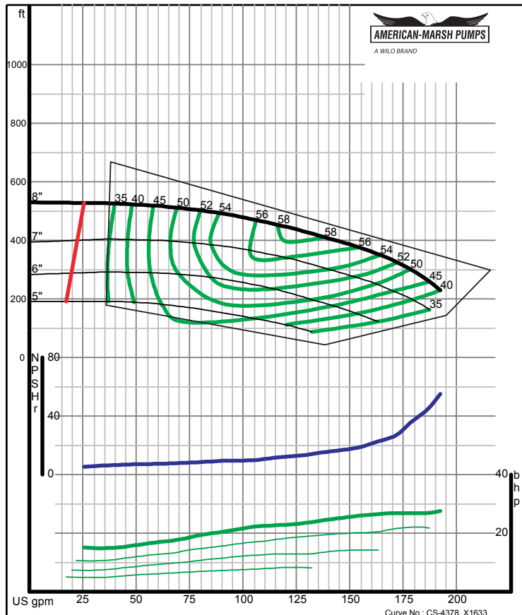
American-Marsh Pumps Size: 1.5x2.5-8 HHM 2 stg Speed: 3500 rpm
