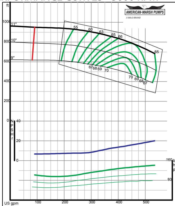
American-Marsh Pumps Size: 3x4-11 HH 2 stages Speed: 3500 rpm
