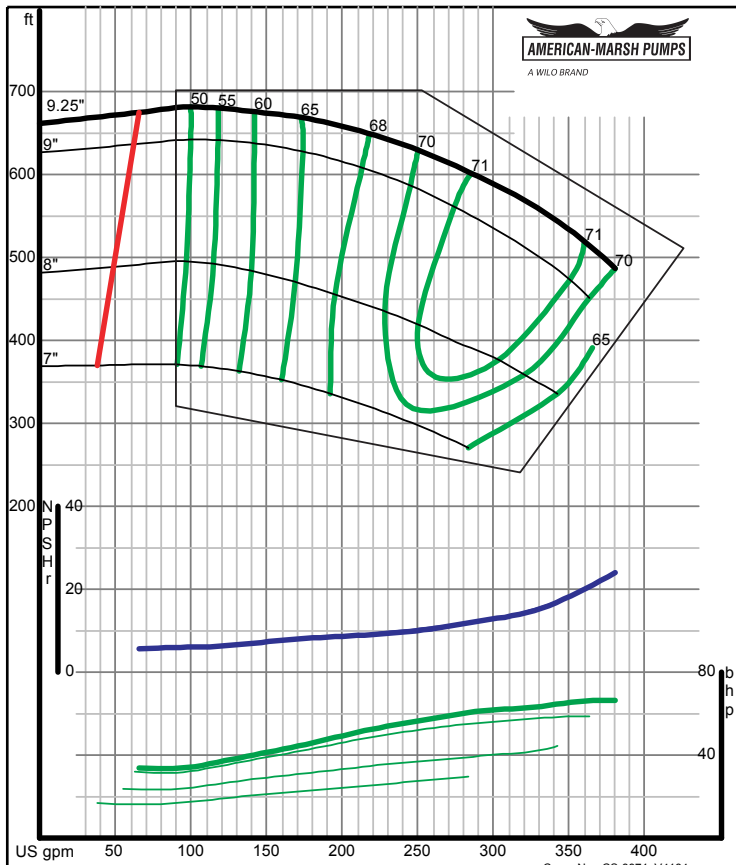
American-Marsh Pumps Size: 2.5x3-9 HH 2 stg Speed: 3500 rpm
