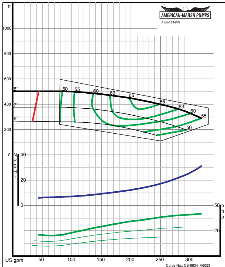
American-Marsh Pumps Size: 2x3-8 HH 2 stg Speed: 3500 rpm
