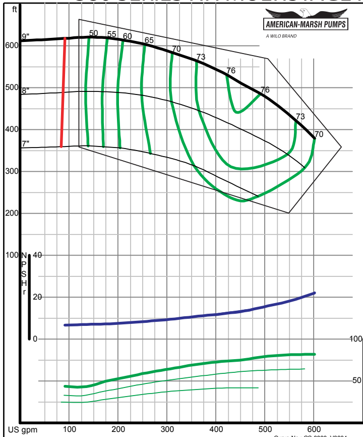
American-Marsh Pumps Size: 3x4-9 HH 2 stg Speed: 3500 rpm
