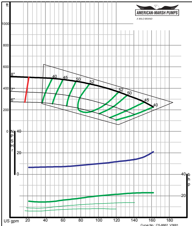
American-Marsh Pumps Size: 1.5x2.5-8 HH 2 stg Speed: 3500 rpm
