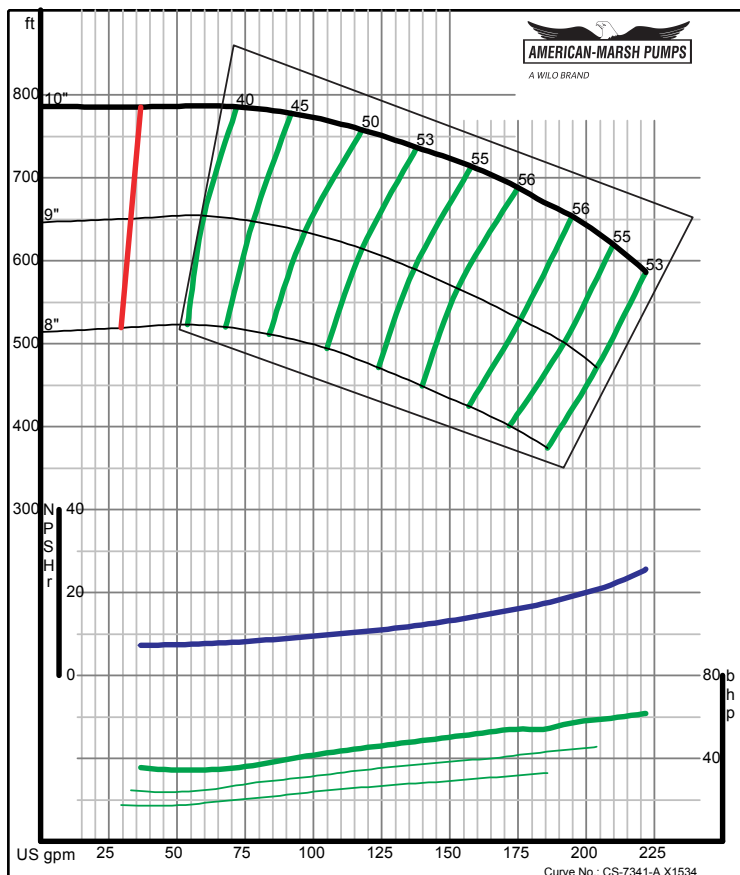
American-Marsh Pumps Size: 1.5x2.5-10 HH 2 stg Speed: 3500 rpm
