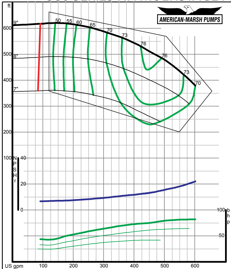
American-Marsh Pumps Size: 3x4-9 HH 2 stg Speed: 3500 rpm
