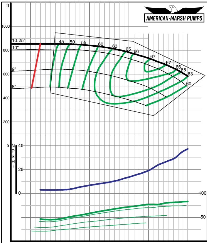
American-Marsh Pumps Size: 2x3-10 HH 2 stg Speed: 3500 rpm
