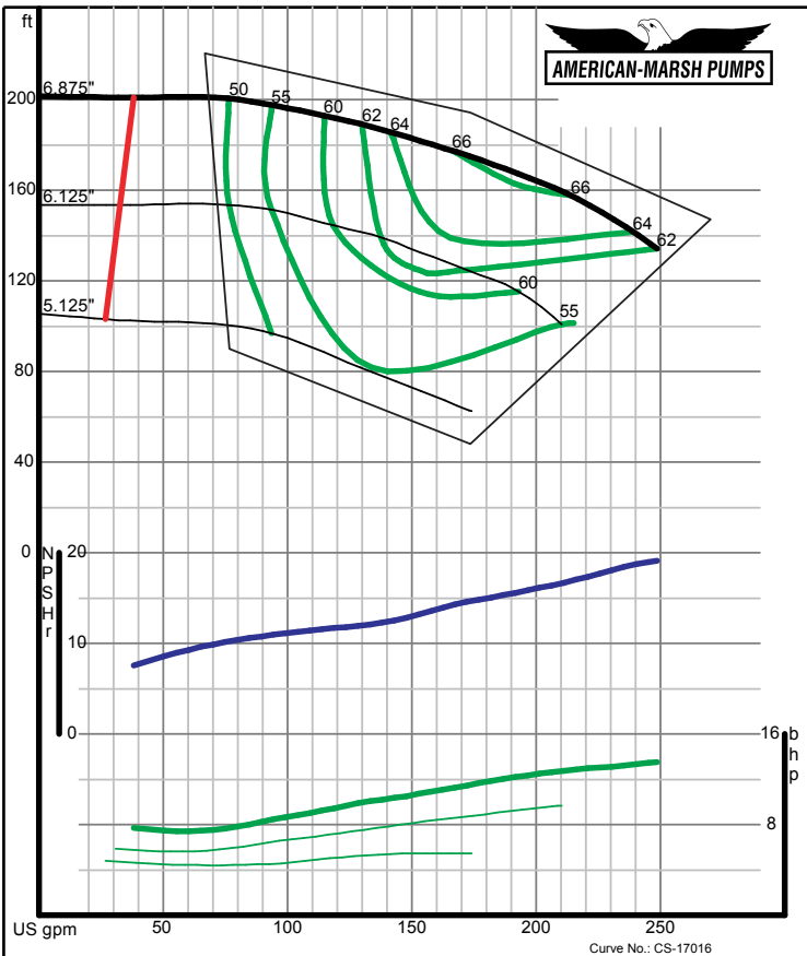
American-Marsh Pumps Size: 2.5x2.5-7A REI Speed: 3500 rpm
