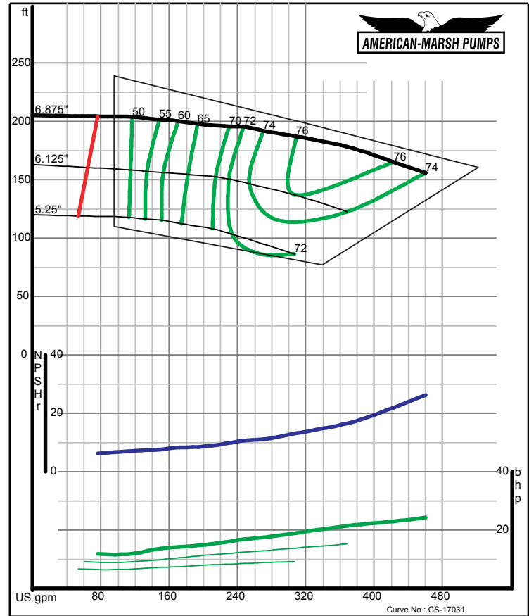
American-Marsh Pumps Size: 2.5x2.5-7B REI Speed: 3500 rpm
