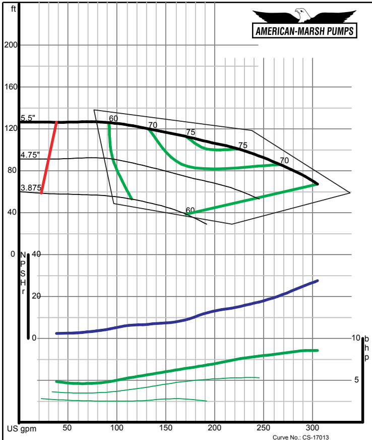
American-Marsh Pumps Size: 2.5x2.5-5A REI Speed: 3500 rpm
