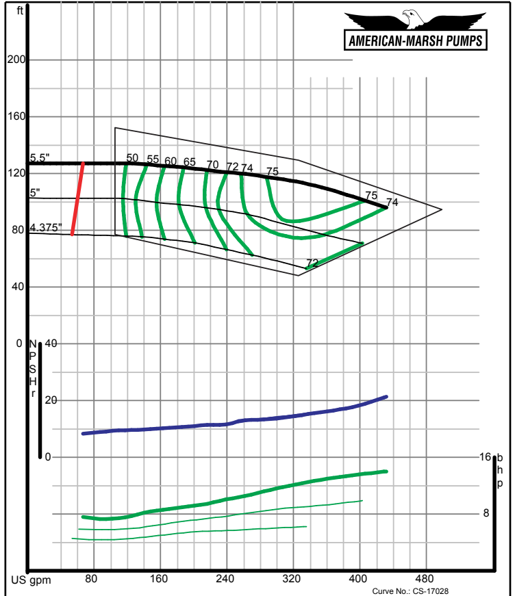
American-Marsh Pumps Size: 2.5x2.5-5B REI Speed: 3500 rpm
