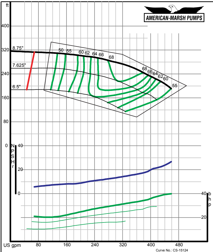
American-Marsh Pumps Size: 2x2.5-8 RE Speed: 3500 rpm
