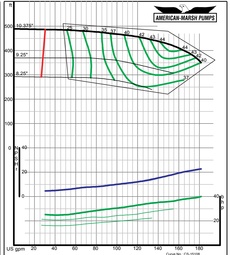
American-Marsh Pumps Size: 1.25x2-10 RE Speed: 3500 rpm 09/03/02
