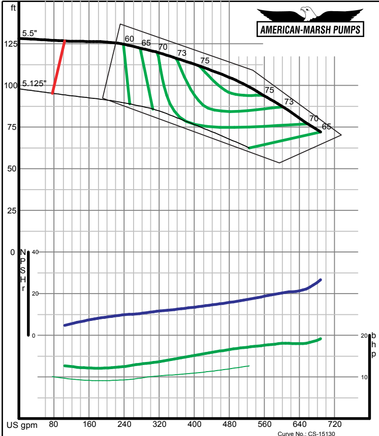
American-Marsh Pumps Size: 2.5x3-5 RE Speed: 3500 rpm
