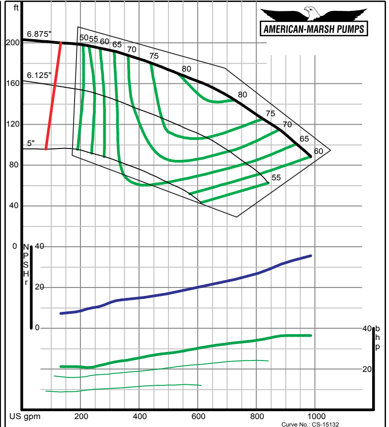
American-Marsh Pumps Size: 2.5x3-7 RE Speed: 3500 rpm
