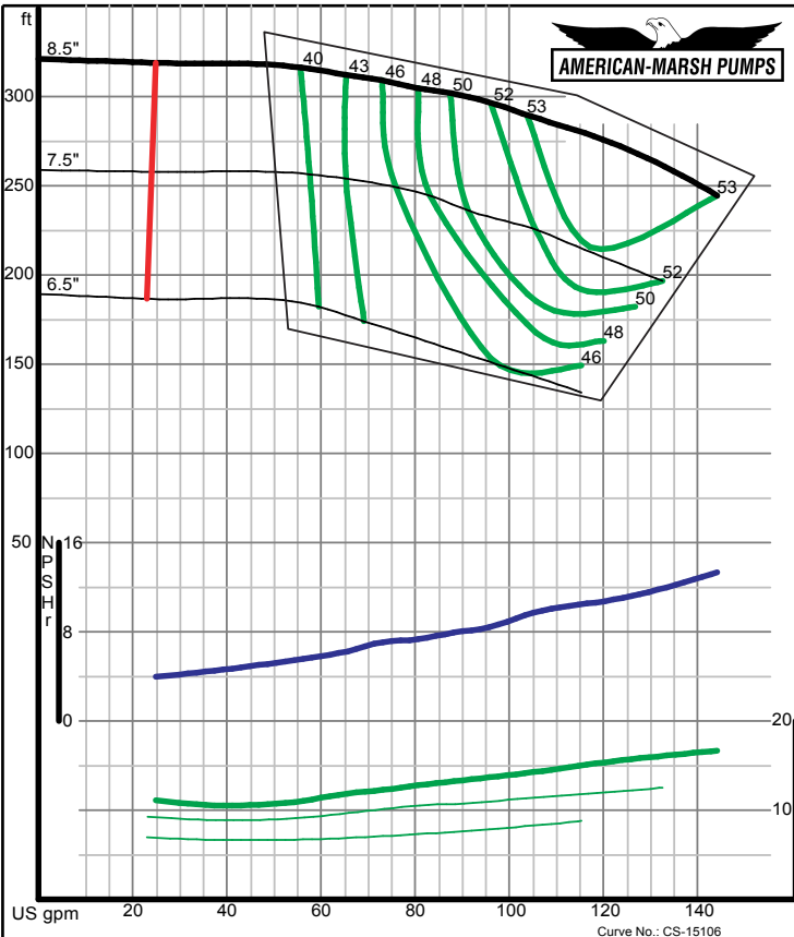
American-Marsh Pumps Size: 1.25x2-8 RE Speed: 3500 rpm 09/03/02
