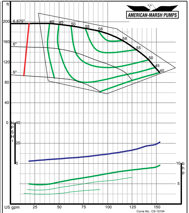
American-Marsh Pumps Size: 1.25x2-7 RE Speed: 3500 rpm 09/03/02
