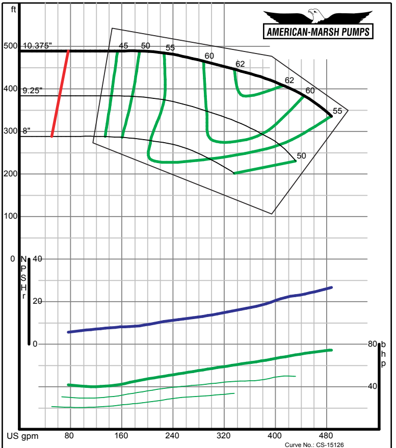
American-Marsh Pumps Size: 2x2.5-10 RE Speed: 3500 rpm
