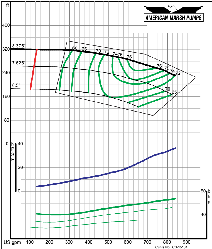
American-Marsh Pumps Size: 2.5x3-8 RE Speed: 3500 rpm
