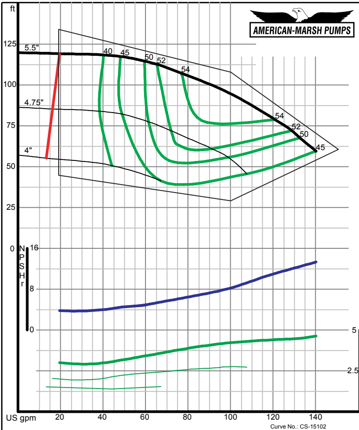
American-Marsh Pumps Size: 1.25x2-5 RE Speed: 3500 rpm 09/03/02
