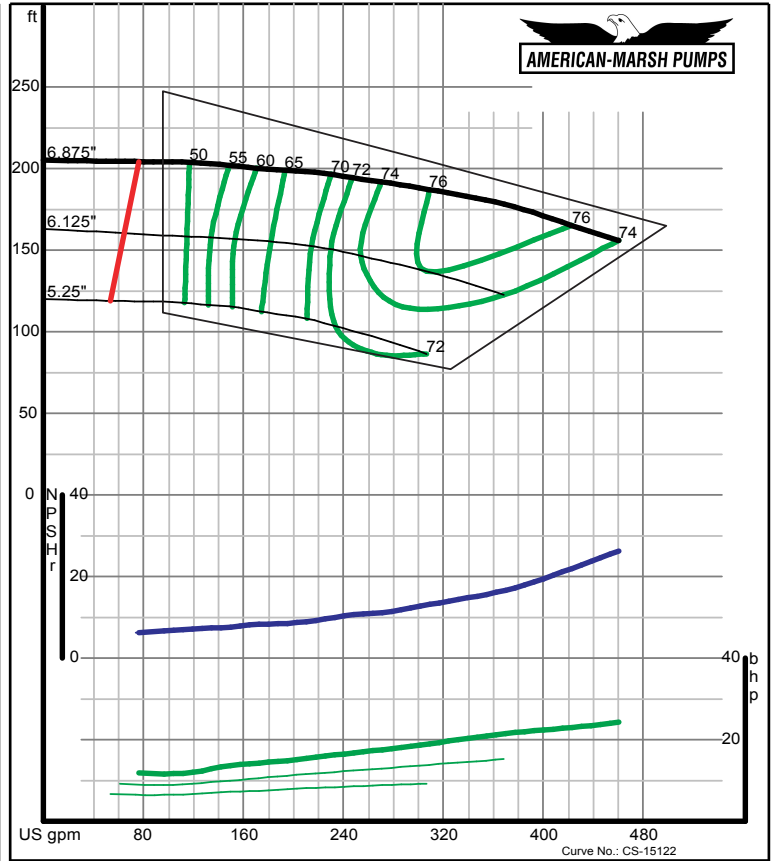
American-Marsh Pumps Size: 2x2.5-7 RE Speed: 3500 rpm
