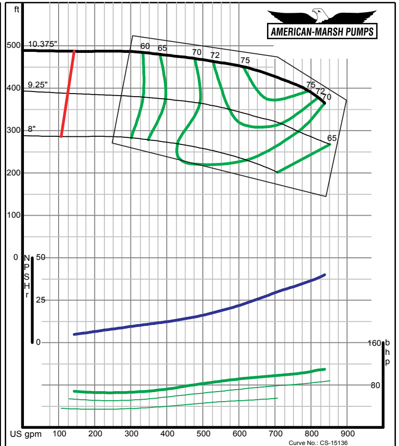
American-Marsh Pumps Size: 2.5x3-10 RE Speed: 3500 rpm
