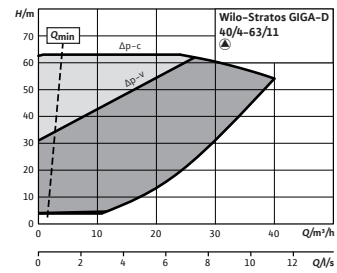
Stratos GIGA-D 40/4-63/11
