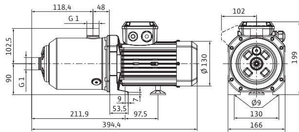
Medana CH1-L.204-1/E/A/10T
