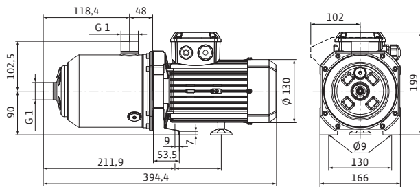
Medana CH1-L.404-2/V/A/10T
