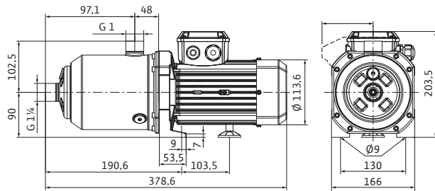
Medana CH1-L.602-1/E/E/10T
