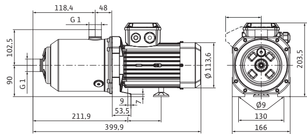
Medana CH1-L.404-2/V/E/10T
