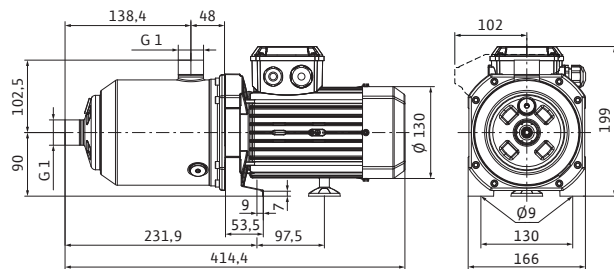
Medana CH1-L.205-2/V/A/10T
