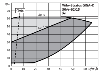
Stratos GIGA-D 50/4-62/15
