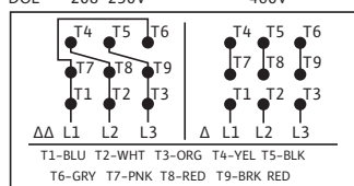
9 Leads 3 to 10 HP, 3600 RPM, TEFC only
