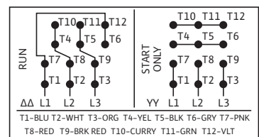
12 Leads above 10 HP, 3600 RPM, TEFC only
