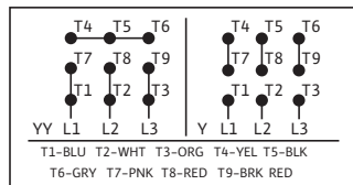
9 Leads up to 2 HP
