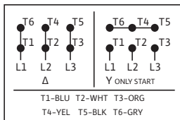
6 Leads up to all
