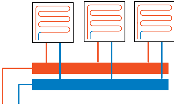
Hall temperature control in an underfloor heating consumer circuit
