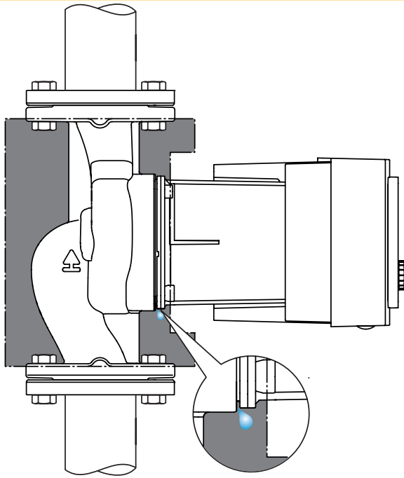
Condensate drain opening in the motor housing
