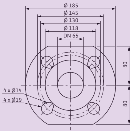
Example combination flange PN 6/10 for 2½ NPS
