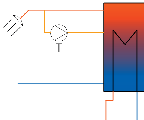
Temperature control of the domestic hot water circulator
