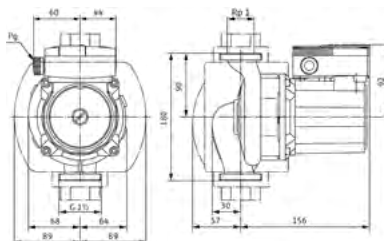
TOP-S 25/10
