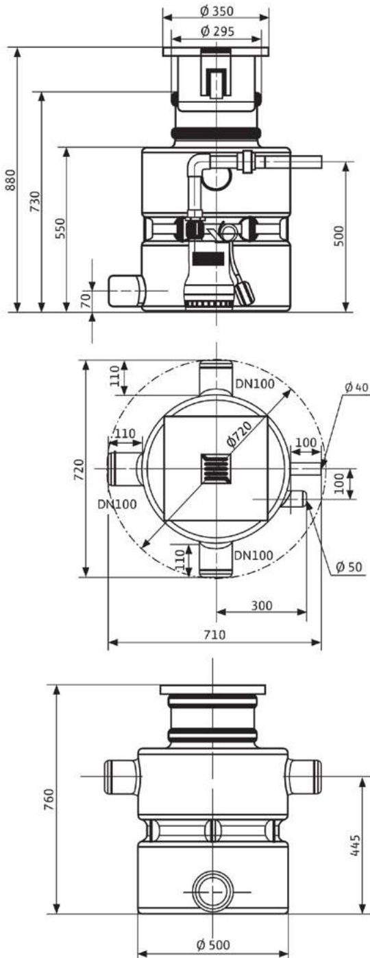
Wilo-DrainLift Box 32
