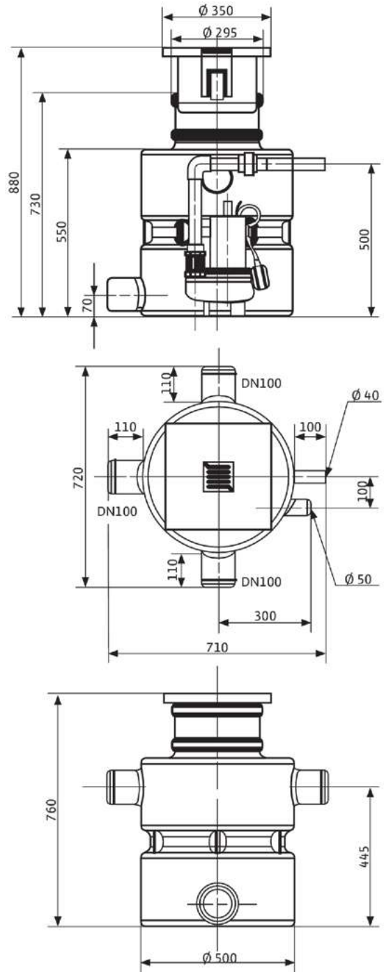
Wilo-DrainLift Box 40
