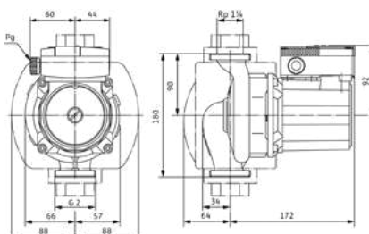
TOP-S 30/5-30/7
