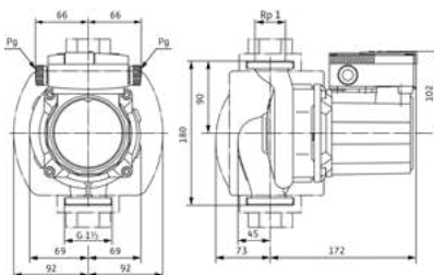
TOP-S 30/5-30/7
