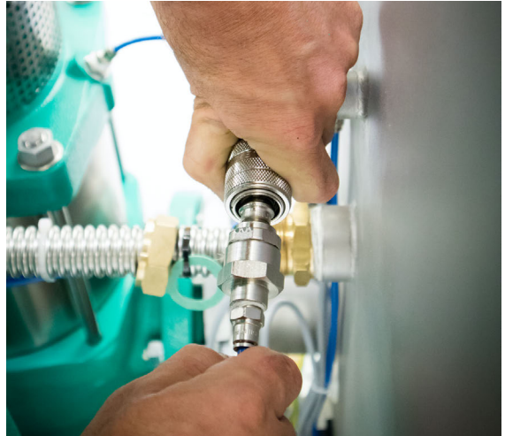
Connection of pump vents to quick-release couplings tank.
