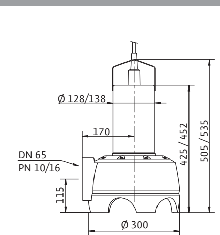
Wilo-Drain TP 65...
