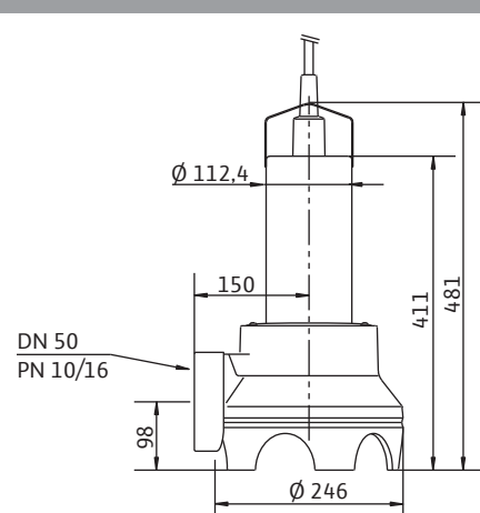
Wilo-Drain TP 50...
