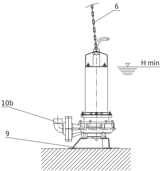
Fig.3: MTS 40/21...39, DN 40 (R1 ½)
