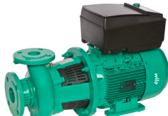
Wilo-CronoBloc-BL-E Q max. 380 m³/h H max. 84 m
