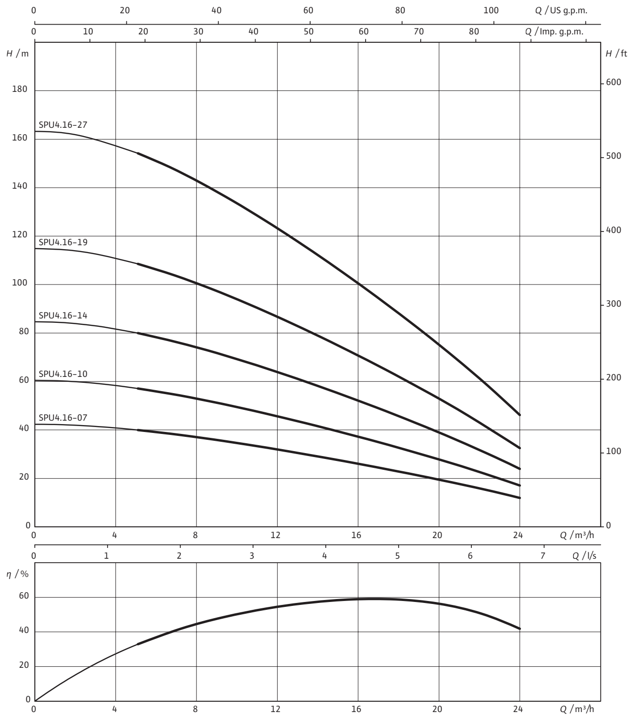
Pump curves FIRST-SPU4.16
